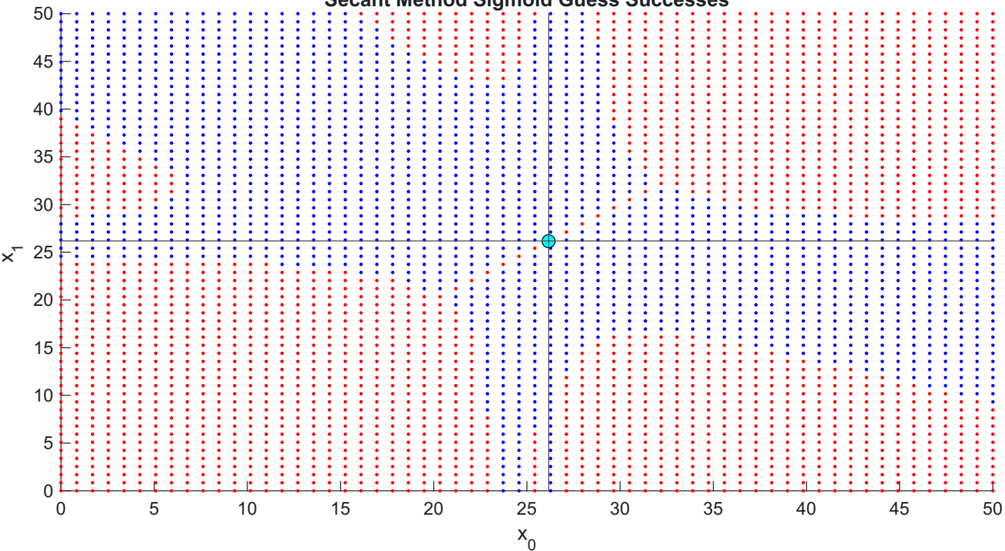
Secant Method Sigmoid Guess Successes
